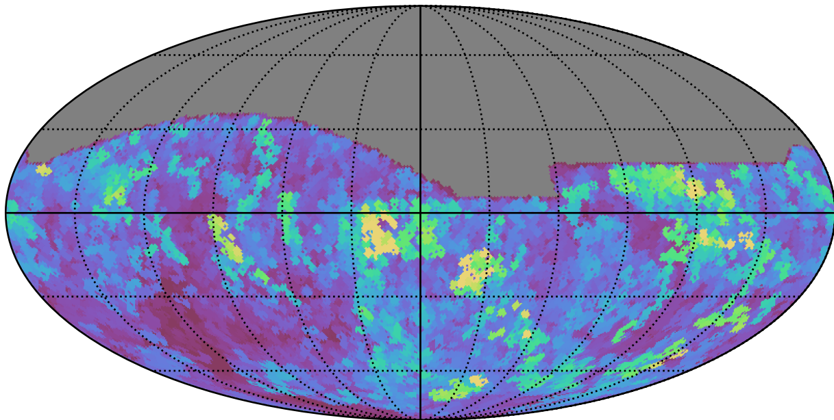
ddf_loaded_fl1_v3.4_10yrs All sky i band: Max seeingEff
