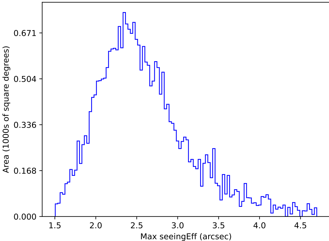
ddf_loaded_fl1_v3.4_10yrs All sky i band: Max seeingEff
