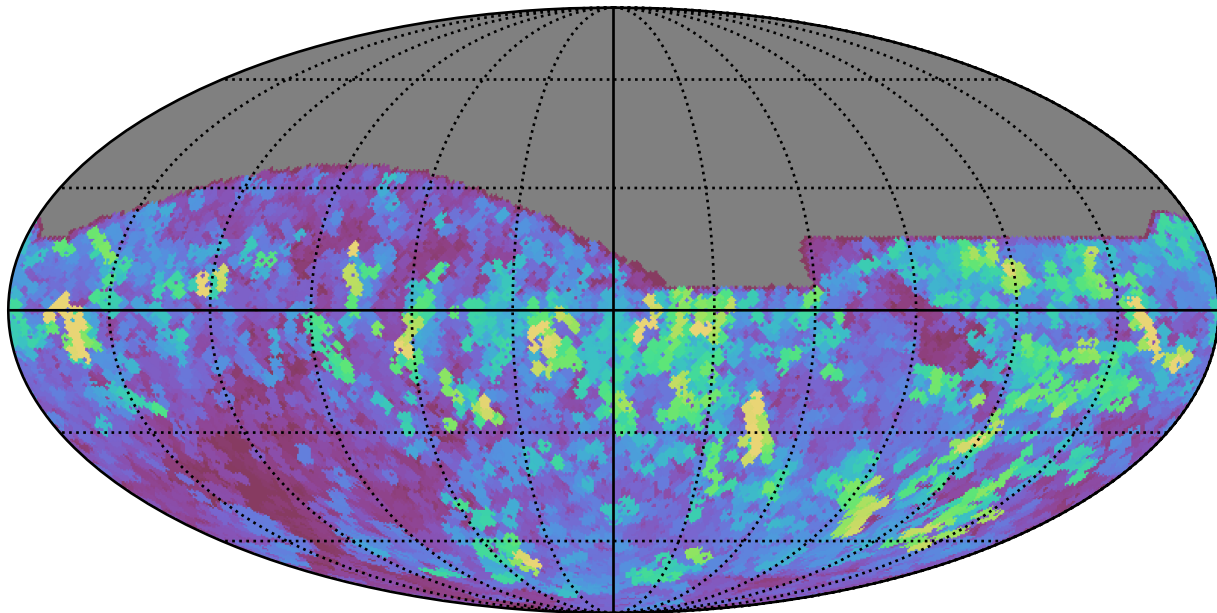
ddf_loaded_fl1_v3.4_10yrs All sky all bands: Max seeingEff
