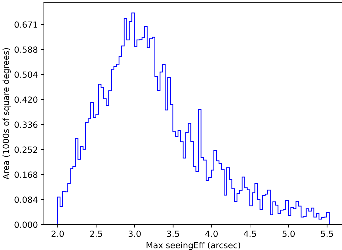
ddf_loaded_fl1_v3.4_10yrs All sky all bands: Max seeingEff
