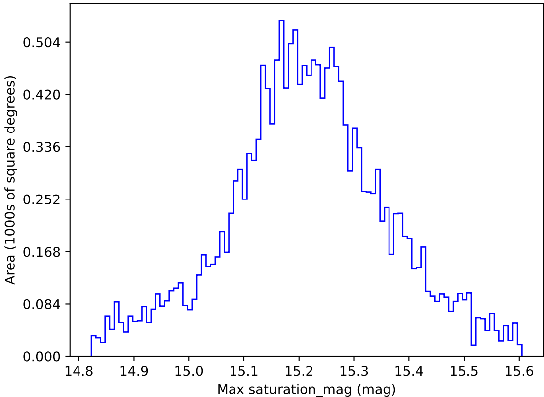
ddf_loaded_fl1_v3.4_10yrs WFD z band: Max saturation_mag
