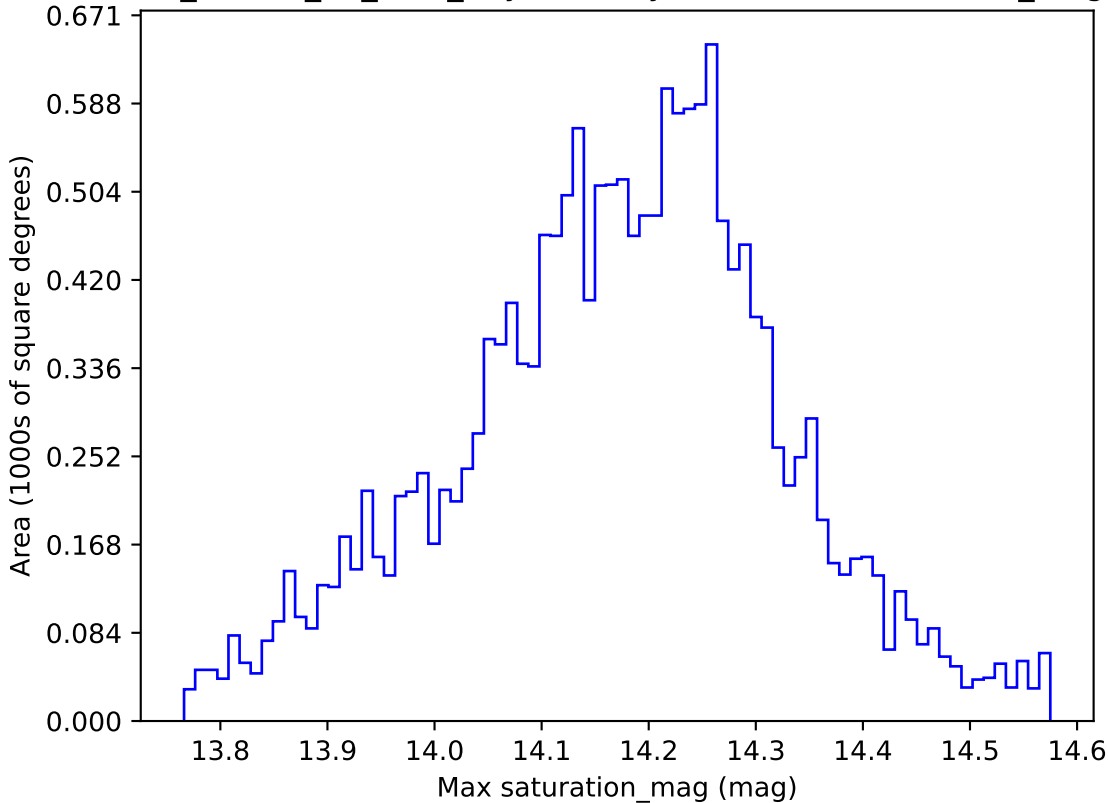
ddf_loaded_fl1_v3.4_10yrs WFD y band: Max saturation_mag
