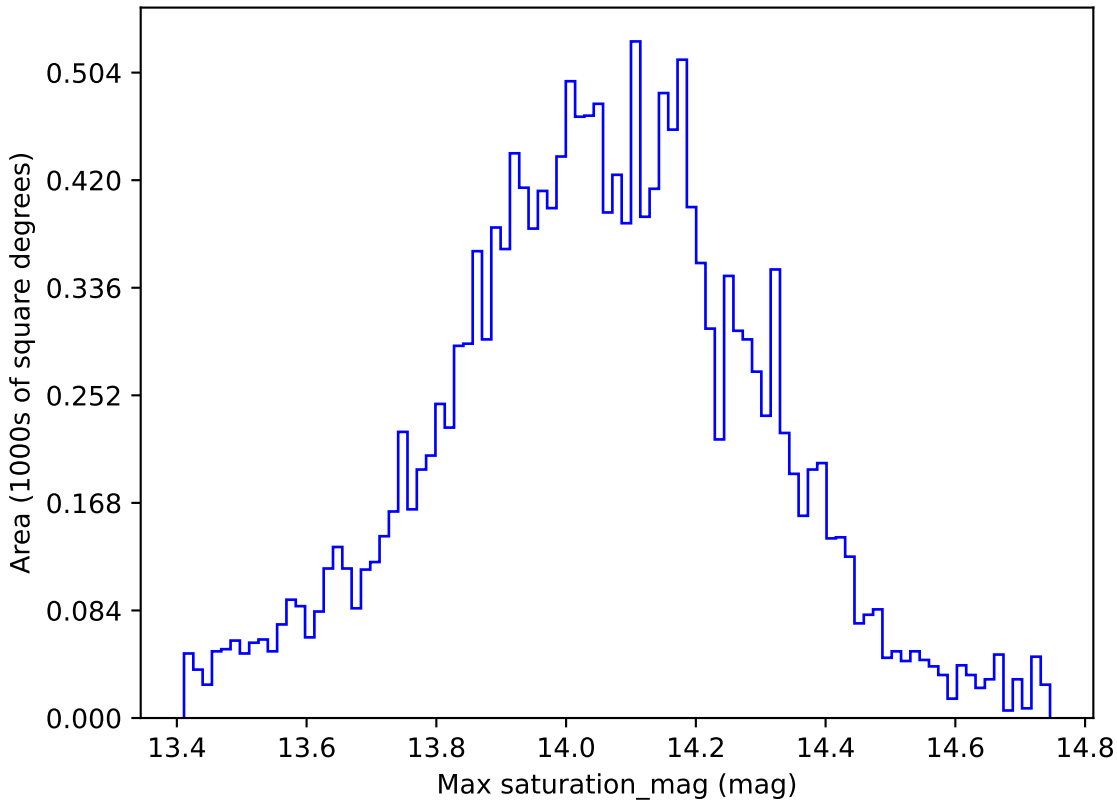
ddf_loaded_fl1_v3.4_10yrs WFD u band: Max saturation_mag
