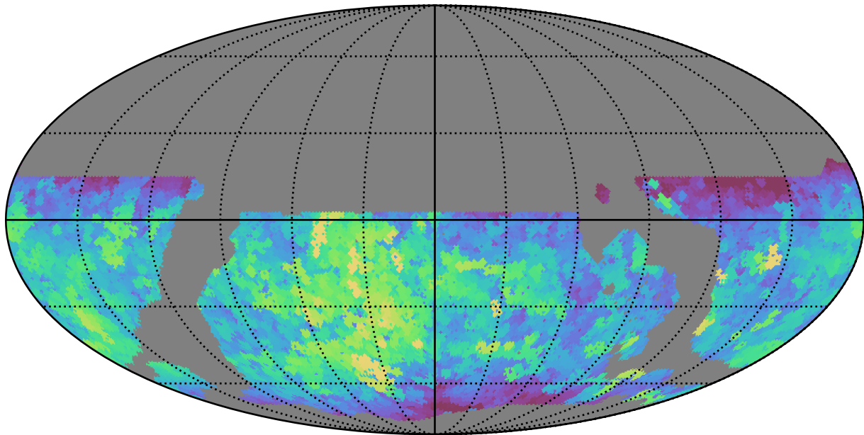
ddf_loaded_fl1_v3.4_10yrs WFD r band: Max saturation_mag
