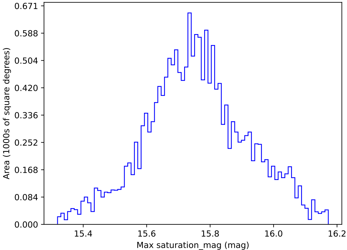
ddf_loaded_fl1_v3.4_10yrs WFD r band: Max saturation_mag
