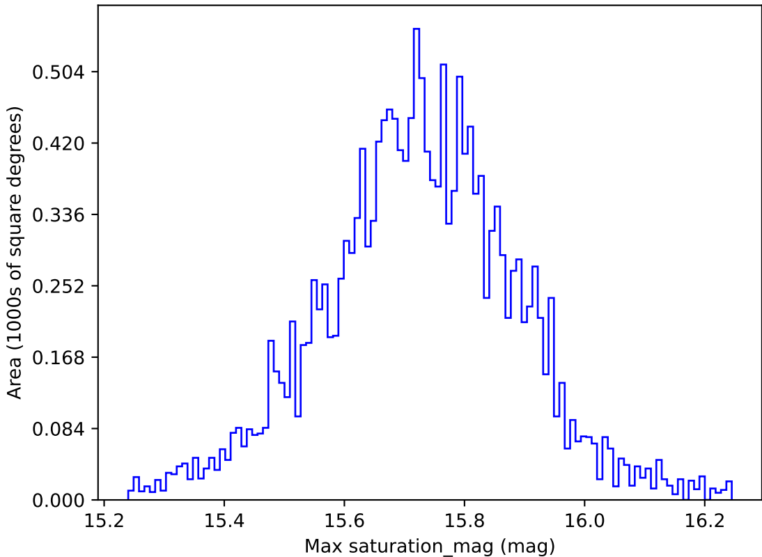
ddf_loaded_fl1_v3.4_10yrs WFD g band: Max saturation_mag
