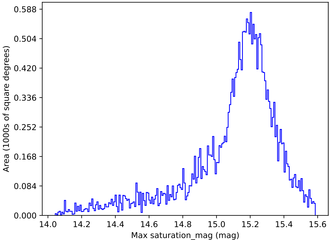
ddf_loaded_fl1_v3.4_10yrs All sky z band: Max saturation_mag
