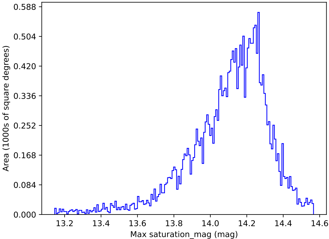
ddf_loaded_fl1_v3.4_10yrs All sky y band: Max saturation_mag
