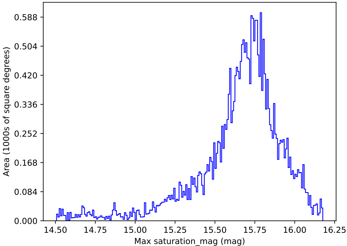
ddf_loaded_fl1_v3.4_10yrs All sky r band: Max saturation_mag
