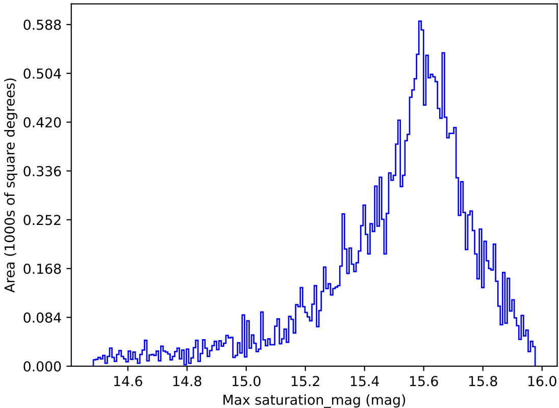
ddf_loaded_fl1_v3.4_10yrs All sky i band: Max saturation_mag
