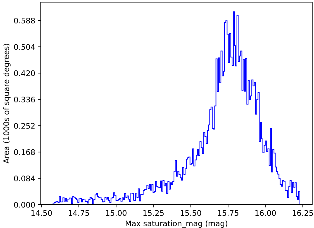
ddf_loaded_fl1_v3.4_10yrs All sky all bands: Max saturation_mag
