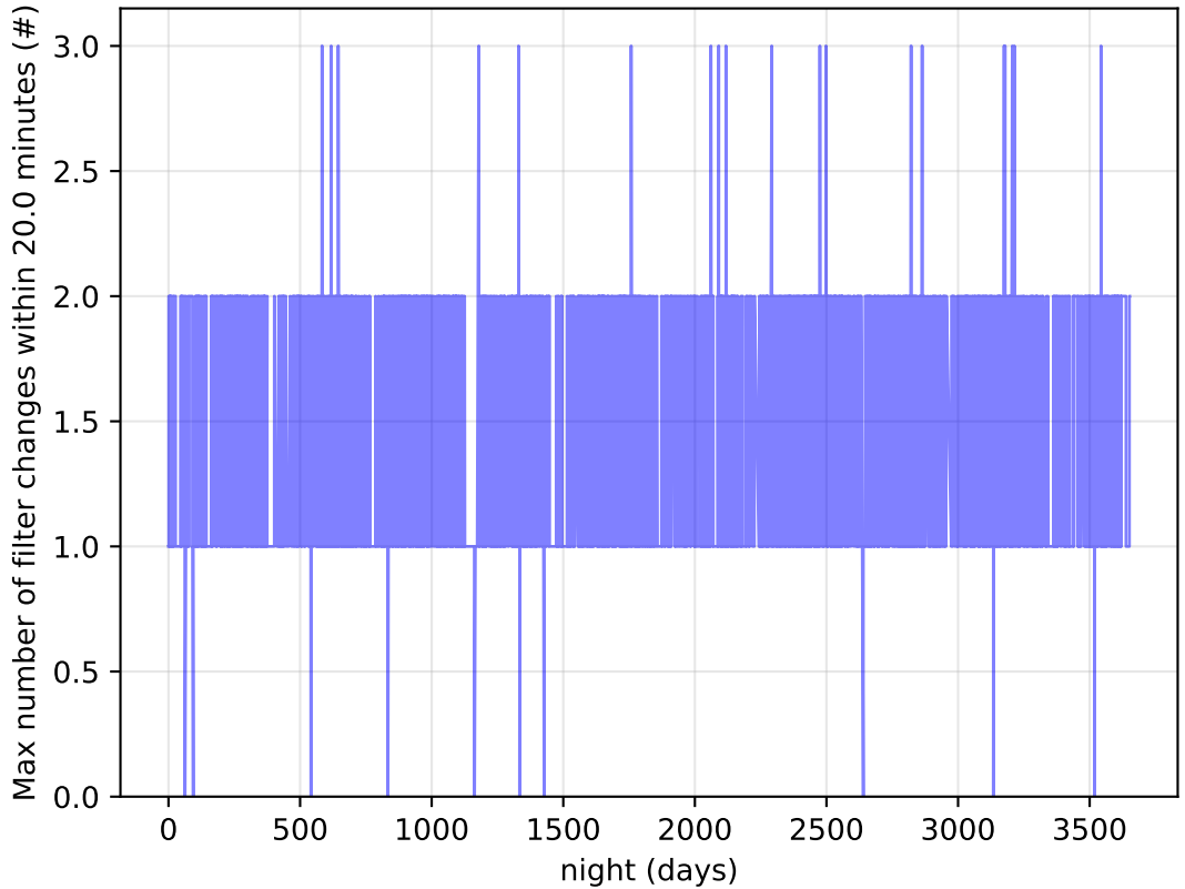
ddf_loaded_fl1_v3.4_10yrs Per Night: Max number of filter changes within 20.0 minutes
