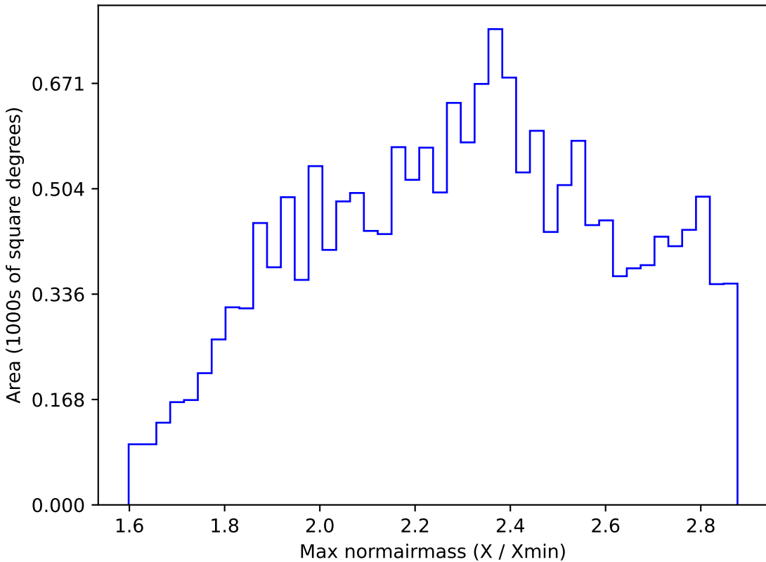
ddf_loaded_fl1_v3.4_10yrs WFD z band: Max normairmass
