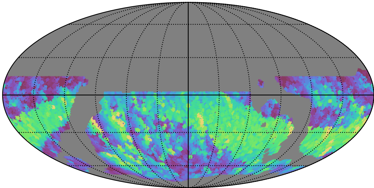
ddf_loaded_fl1_v3.4_10yrs WFD r band: Max normairmass
