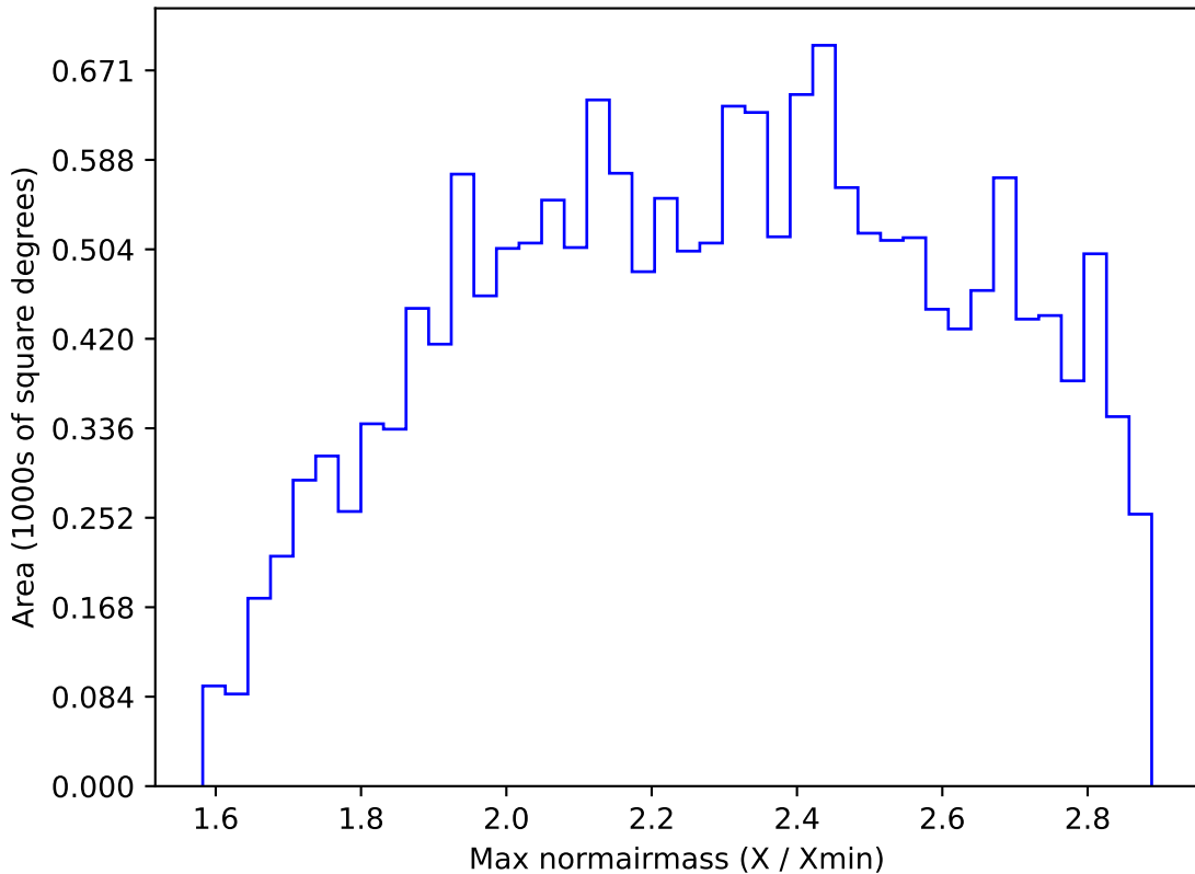
ddf_loaded_fl1_v3.4_10yrs WFD i band: Max normairmass
