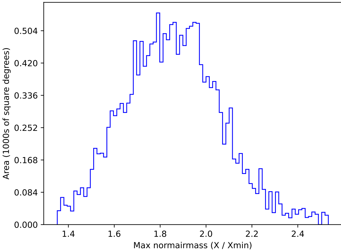
ddf_loaded_fl1_v3.4_10yrs WFD g band: Max normairmass
