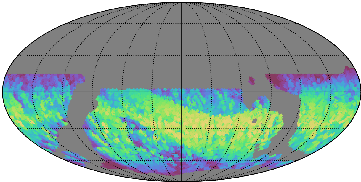
ddf_loaded_fl1_v3.4_10yrs WFD all bands: Max normairmass
