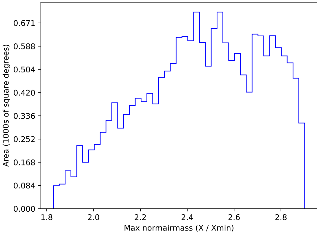
ddf_loaded_fl1_v3.4_10yrs WFD all bands: Max normairmass
