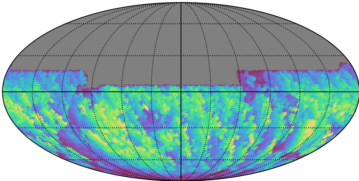
ddf_loaded_fl1_v3.4_10yrs All sky y band: Max normairmass
