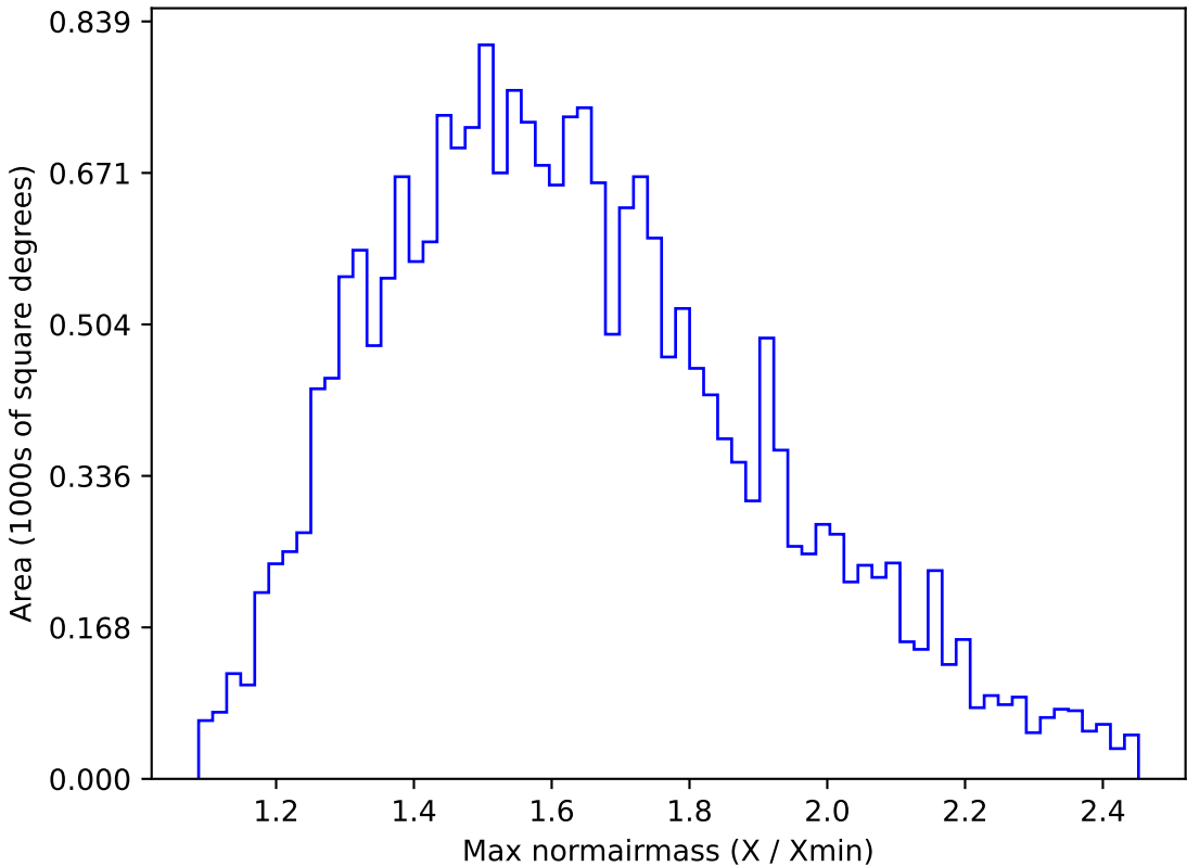
ddf_loaded_fl1_v3.4_10yrs All sky u band: Max normairmass
