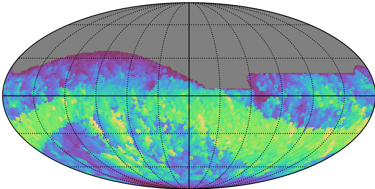
ddf_loaded_fl1_v3.4_10yrs All sky r band: Max normairmass
