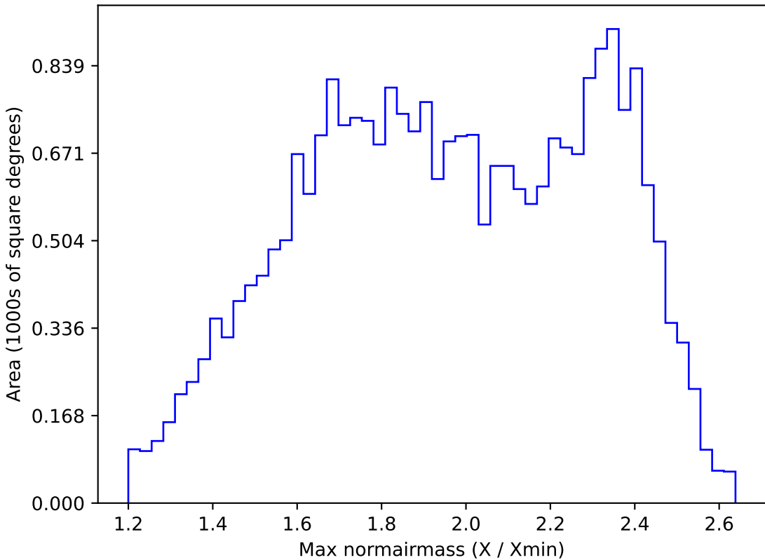
ddf_loaded_fl1_v3.4_10yrs All sky r band: Max normairmass
