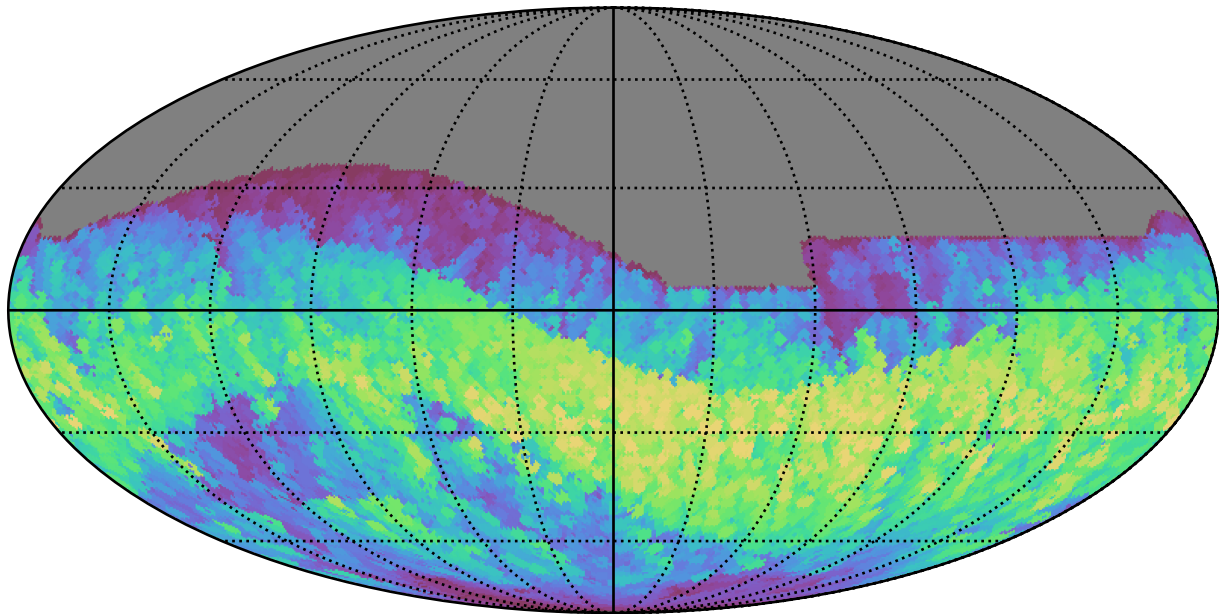
ddf_loaded_fl1_v3.4_10yrs All sky i band: Max normairmass
