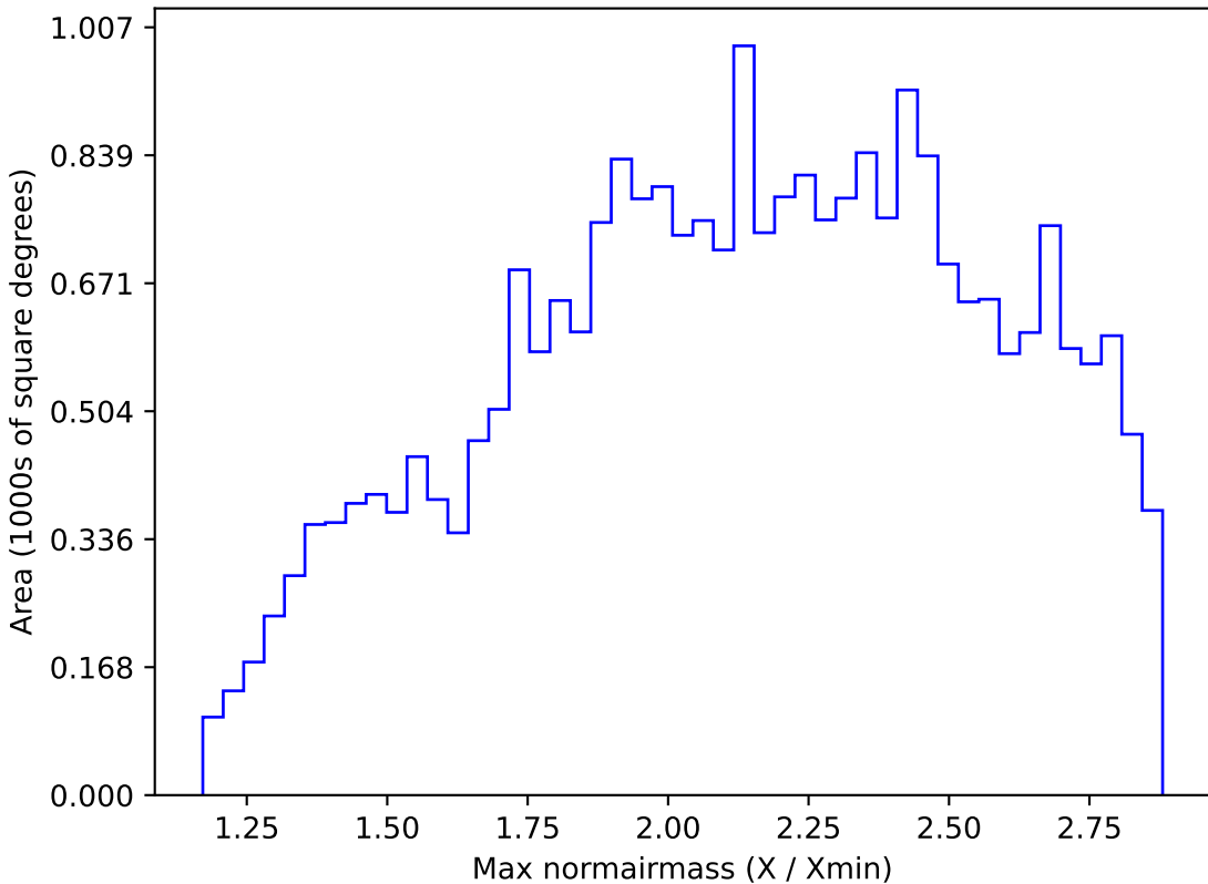
ddf_loaded_fl1_v3.4_10yrs All sky i band: Max normairmass
