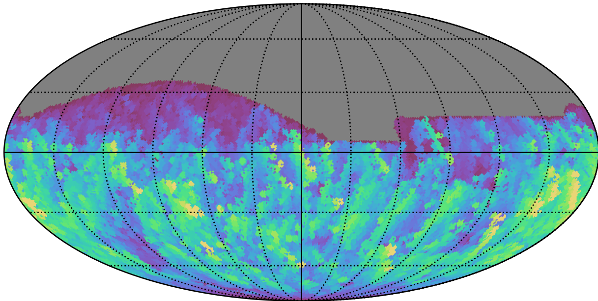
ddf_loaded_fl1_v3.4_10yrs All sky g band: Max normairmass
