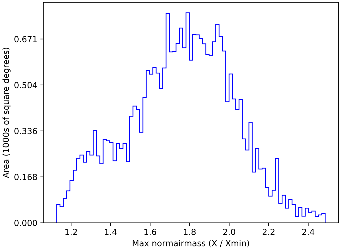
ddf_loaded_fl1_v3.4_10yrs All sky g band: Max normairmass
