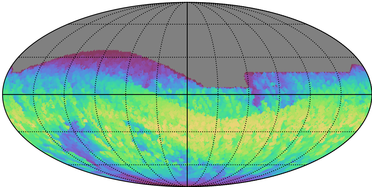
ddf_loaded_fl1_v3.4_10yrs All sky all bands: Max normairmass
