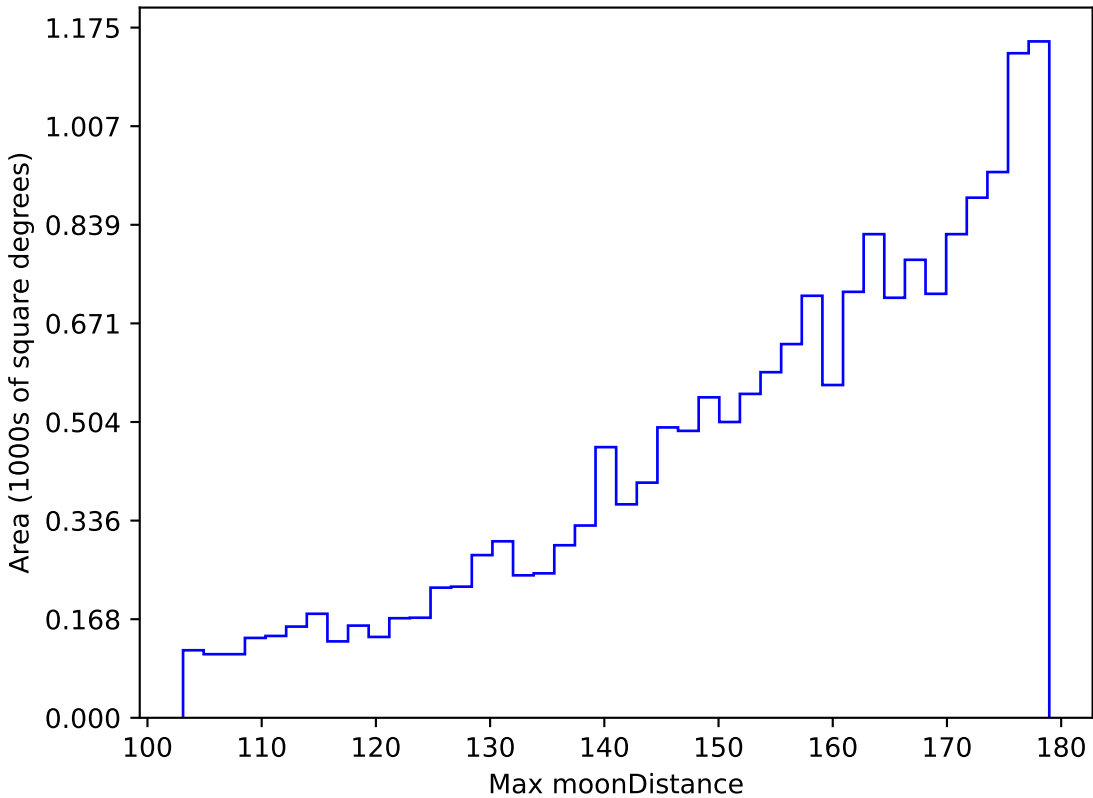
ddf_loaded_fl1_v3.4_10yrs WFD z band: Max moonDistance
