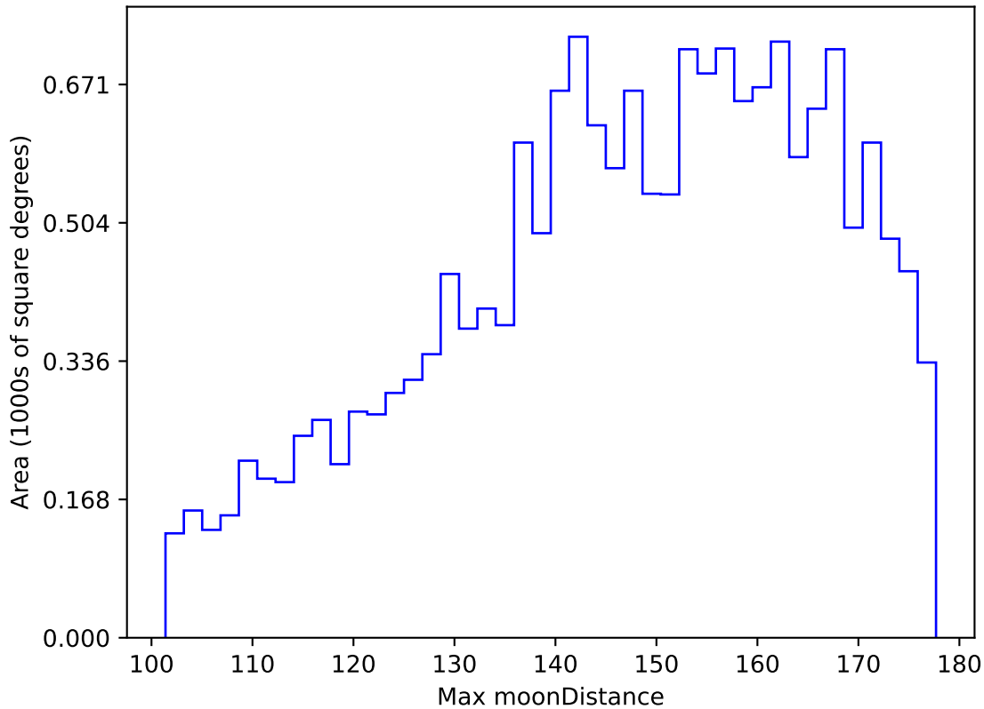
ddf_loaded_fl1_v3.4_10yrs WFD y band: Max moonDistance
