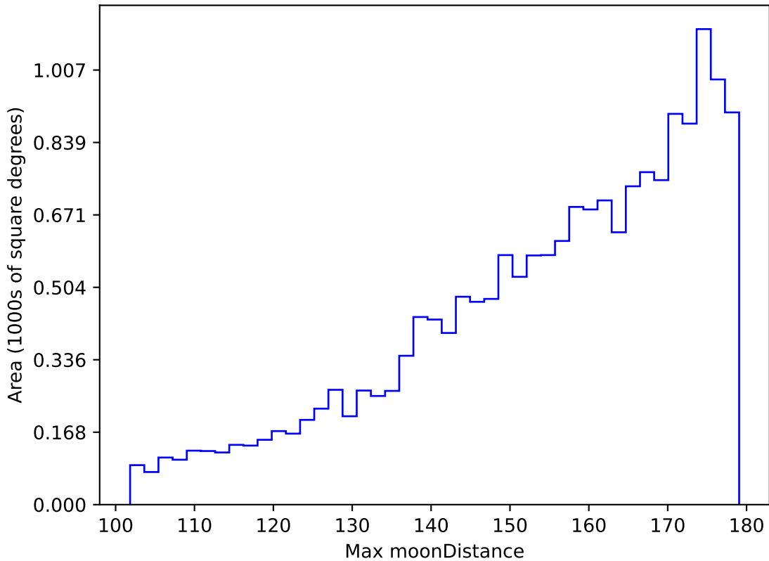
ddf_loaded_fl1_v3.4_10yrs WFD u band: Max moonDistance
