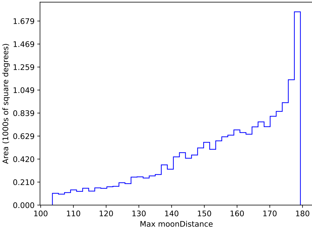
ddf_loaded_fl1_v3.4_10yrs WFD r band: Max moonDistance
