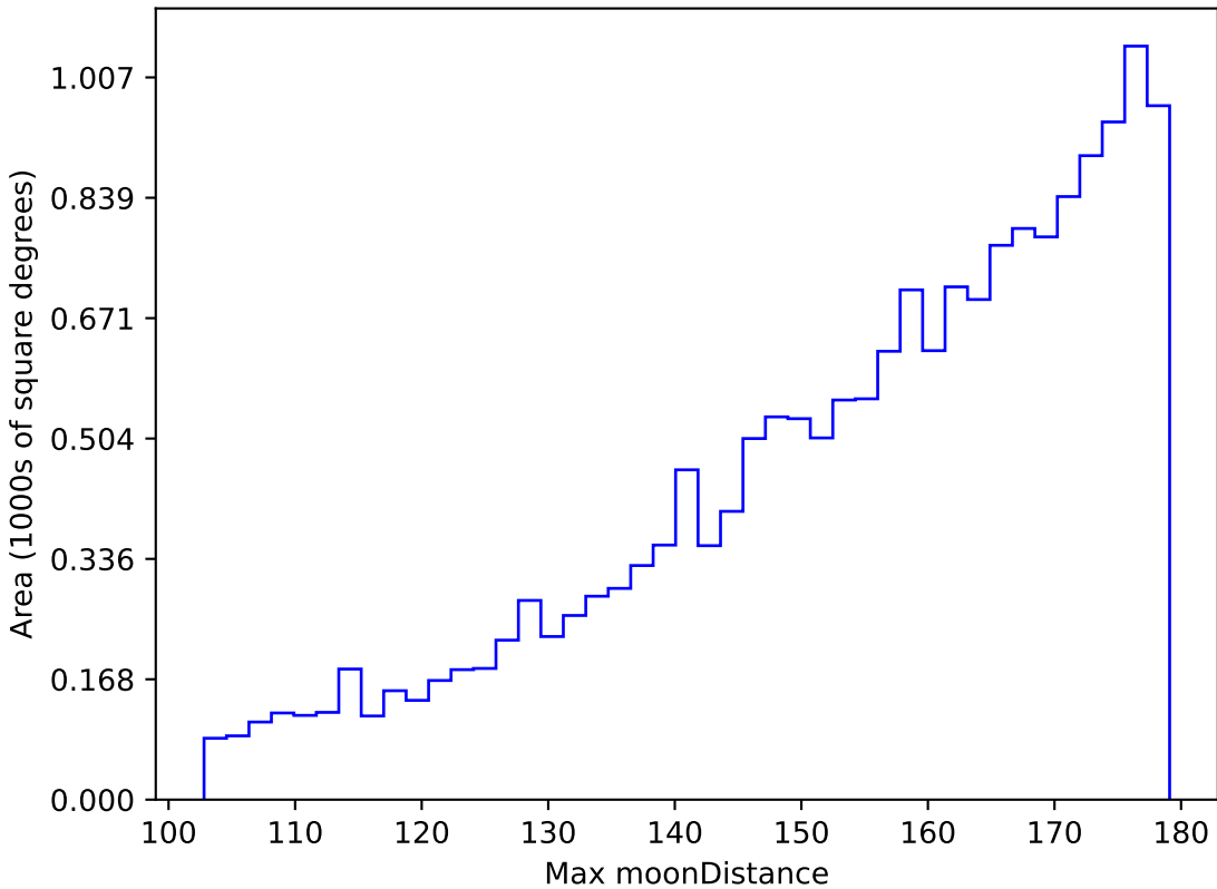
ddf_loaded_fl1_v3.4_10yrs WFD g band: Max moonDistance
