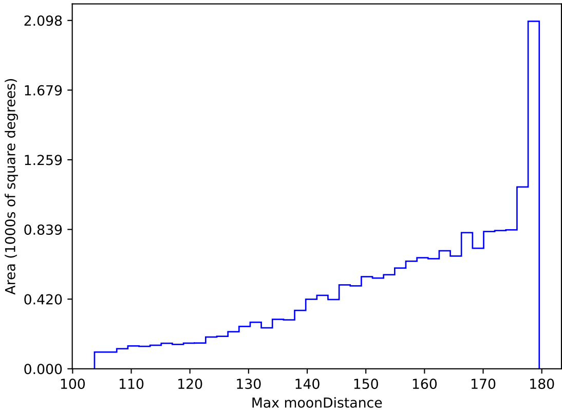
ddf_loaded_fl1_v3.4_10yrs WFD all bands: Max moonDistance
