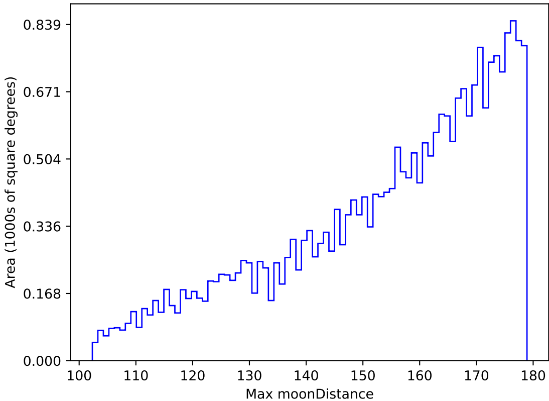
ddf_loaded_fl1_v3.4_10yrs All sky z band: Max moonDistance
