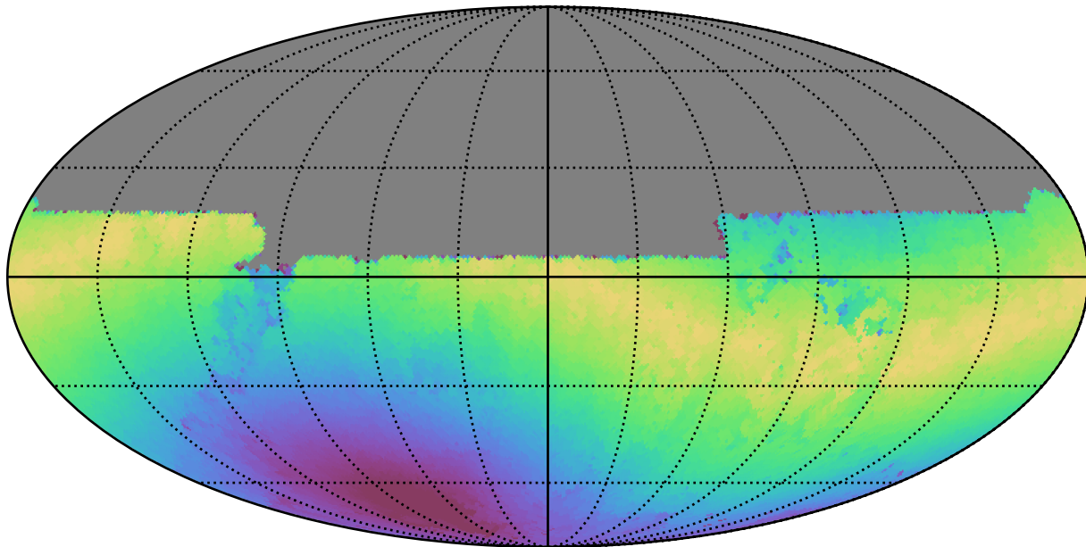
ddf_loaded_fl1_v3.4_10yrs All sky u band: Max moonDistance
