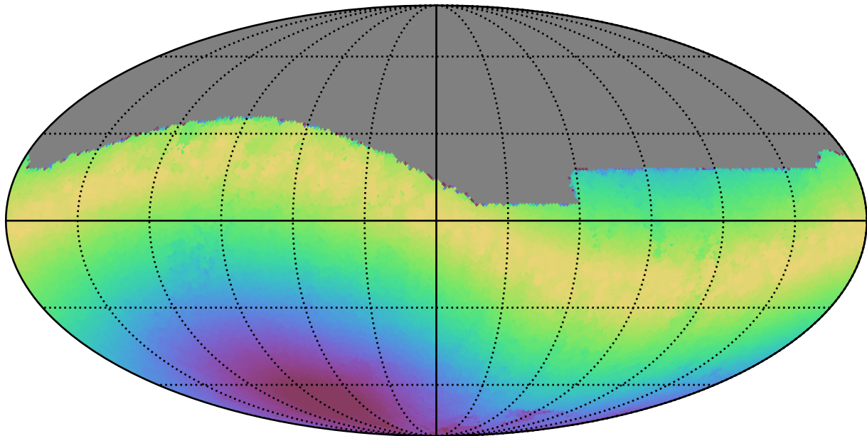
ddf_loaded_fl1_v3.4_10yrs All sky r band: Max moonDistance
