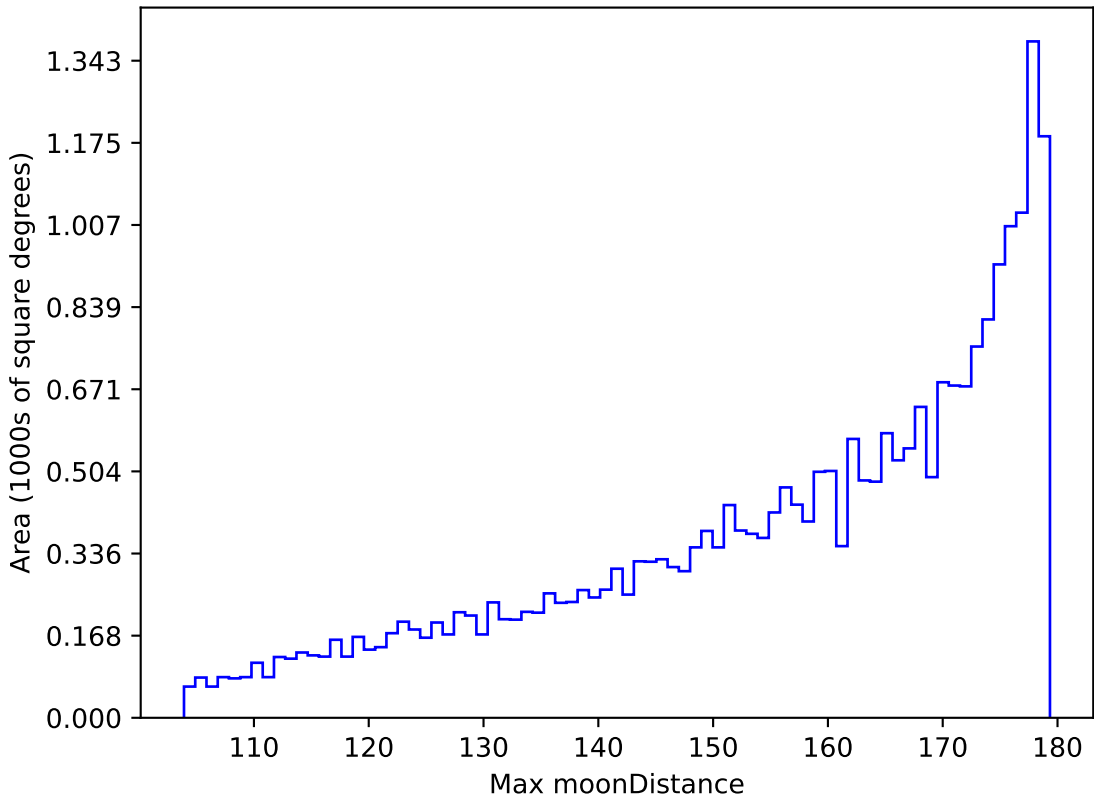
ddf_loaded_fl1_v3.4_10yrs All sky r band: Max moonDistance
