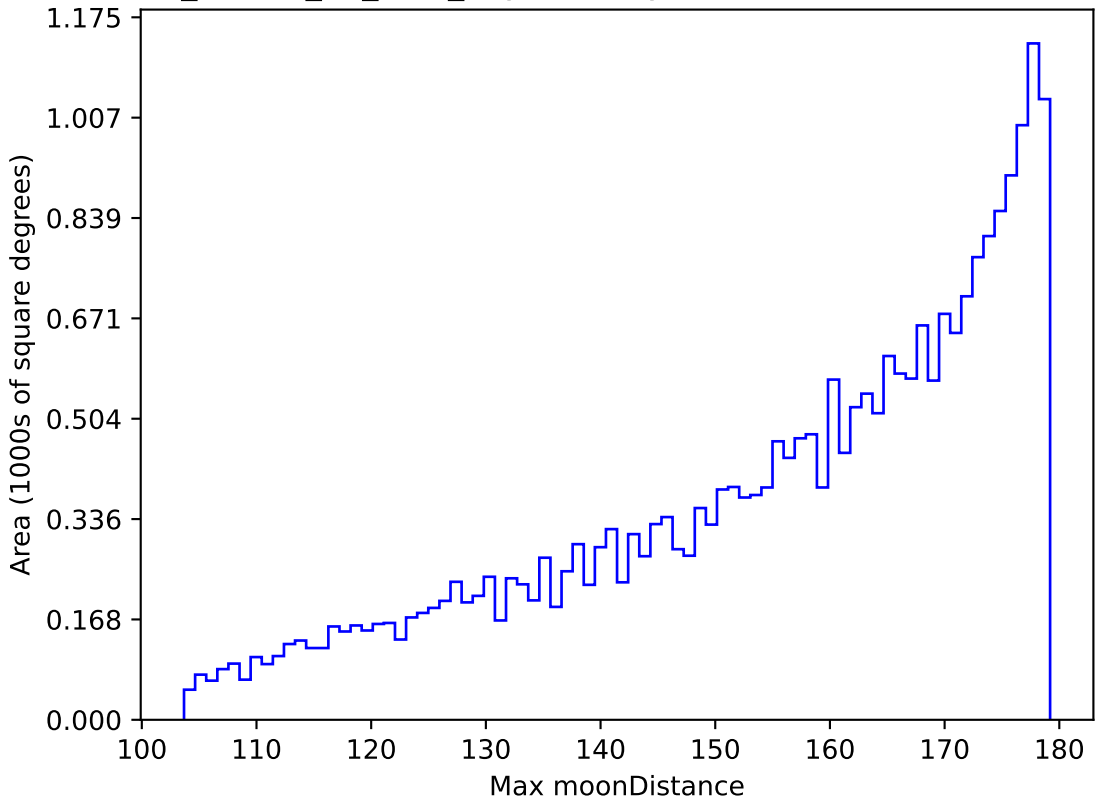
ddf_loaded_fl1_v3.4_10yrs All sky i band: Max moonDistance
