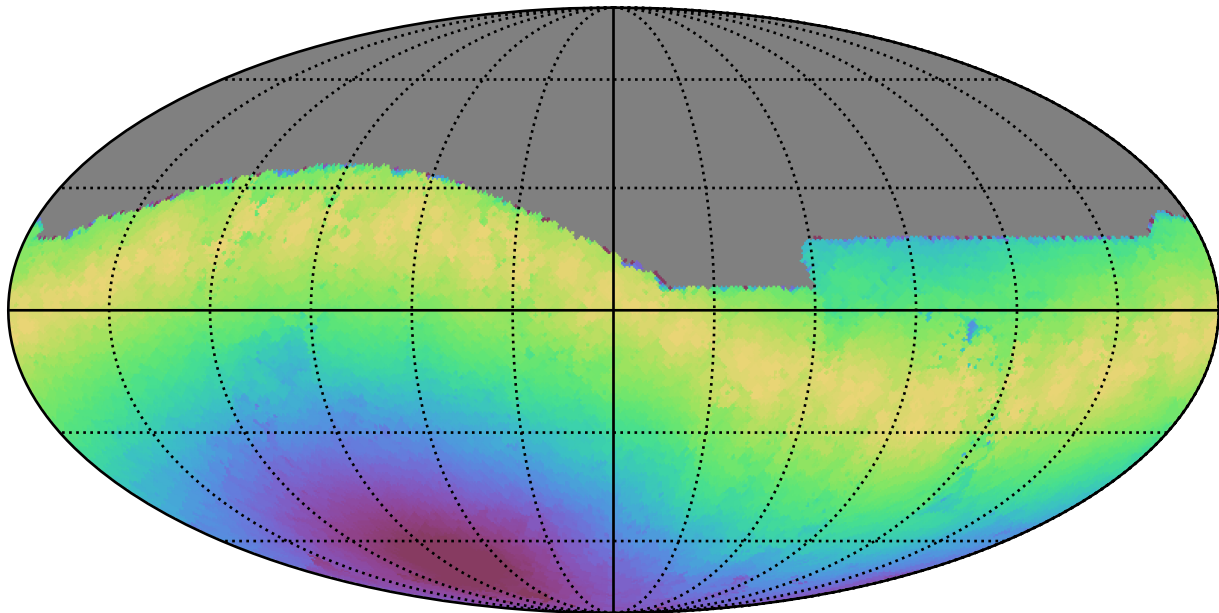
ddf_loaded_fl1_v3.4_10yrs All sky g band: Max moonDistance
