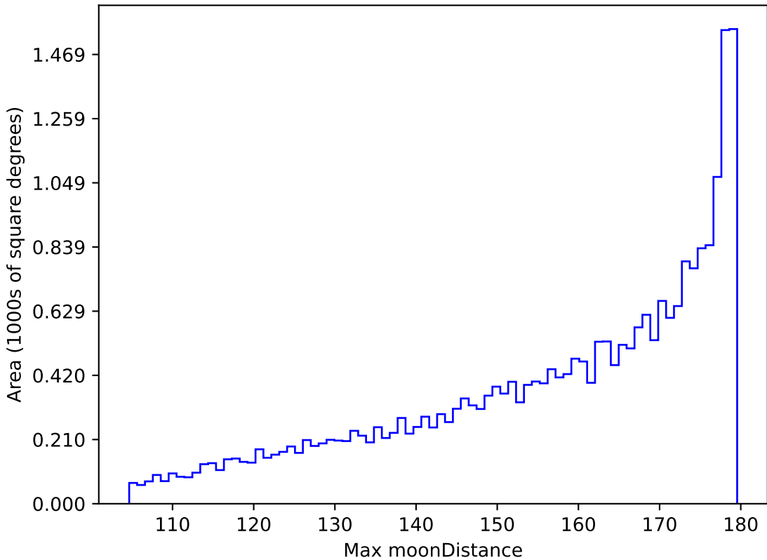
ddf_loaded_fl1_v3.4_10yrs All sky all bands: Max moonDistance
