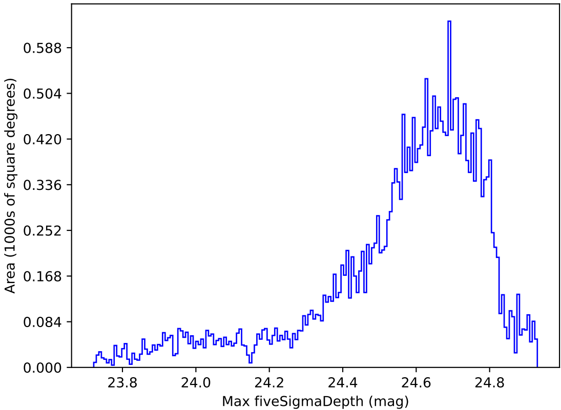
ddf_loaded_fl1_v3.4_10yrs Yr 1 r band: Max fiveSigmaDepth
