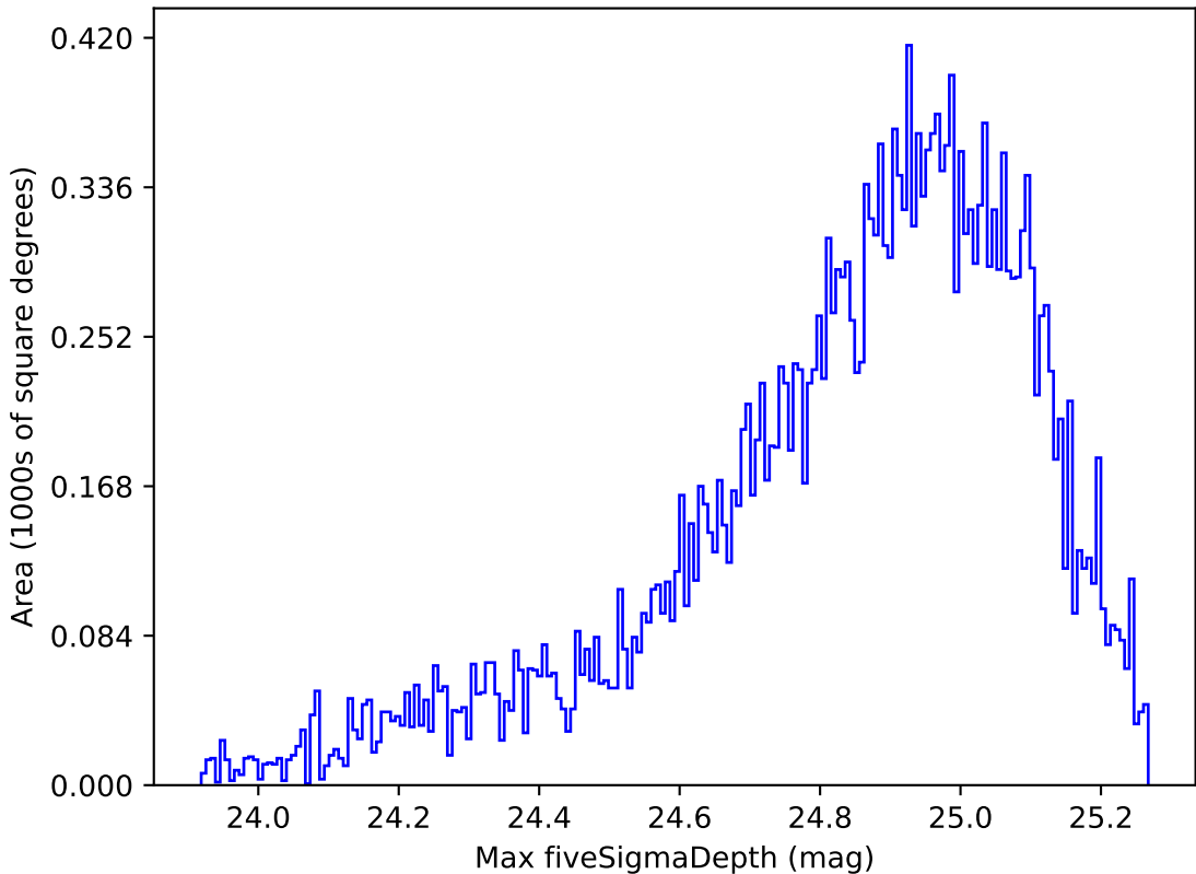
ddf_loaded_fl1_v3.4_10yrs Yr 1 all bands: Max fiveSigmaDepth
