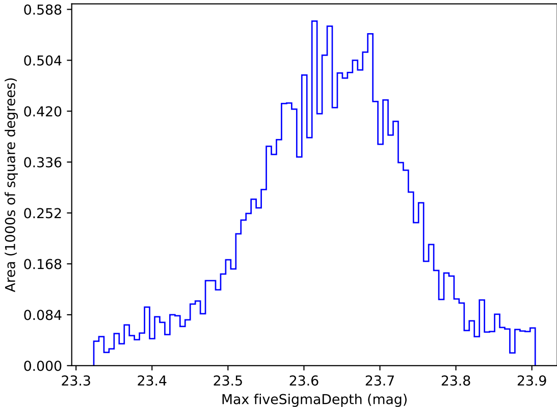
ddf_loaded_fl1_v3.4_10yrs WFD z band: Max fiveSigmaDepth
