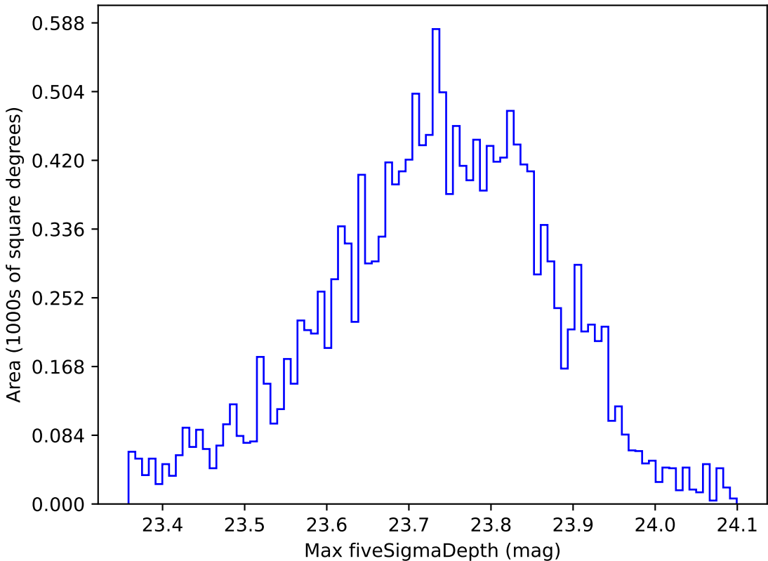
ddf_loaded_fl1_v3.4_10yrs WFD u band: Max fiveSigmaDepth
