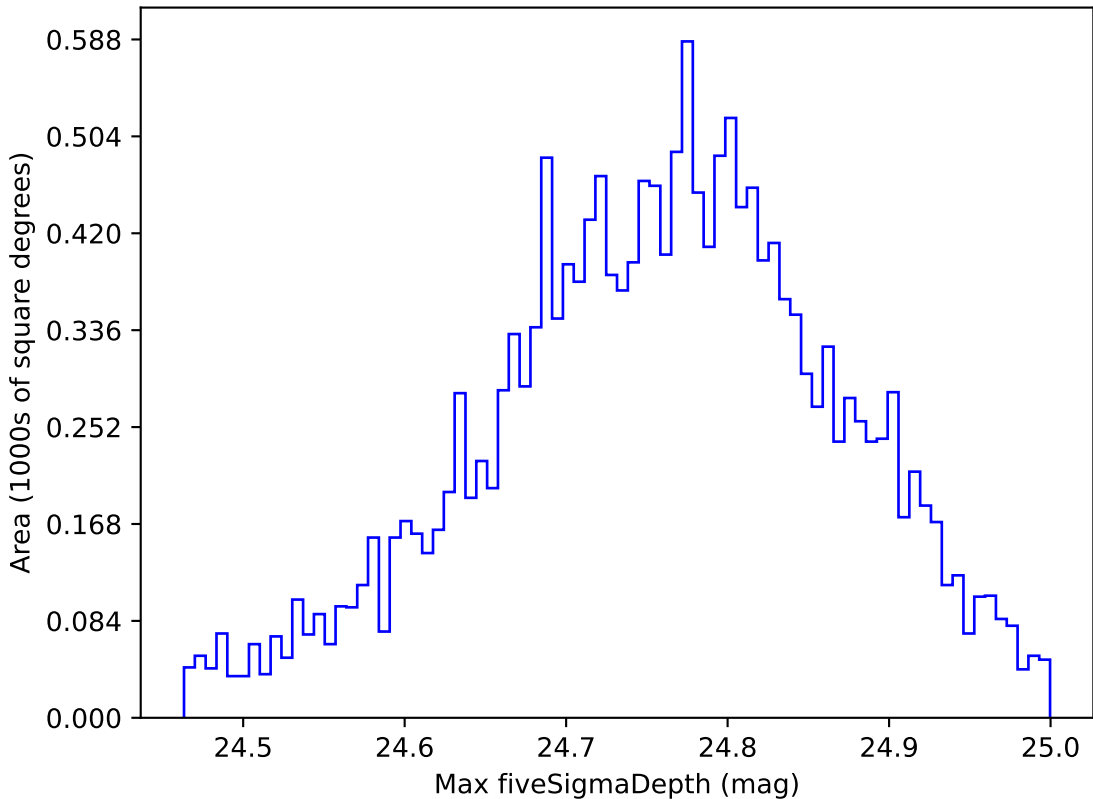
ddf_loaded_fl1_v3.4_10yrs WFD r band: Max fiveSigmaDepth
