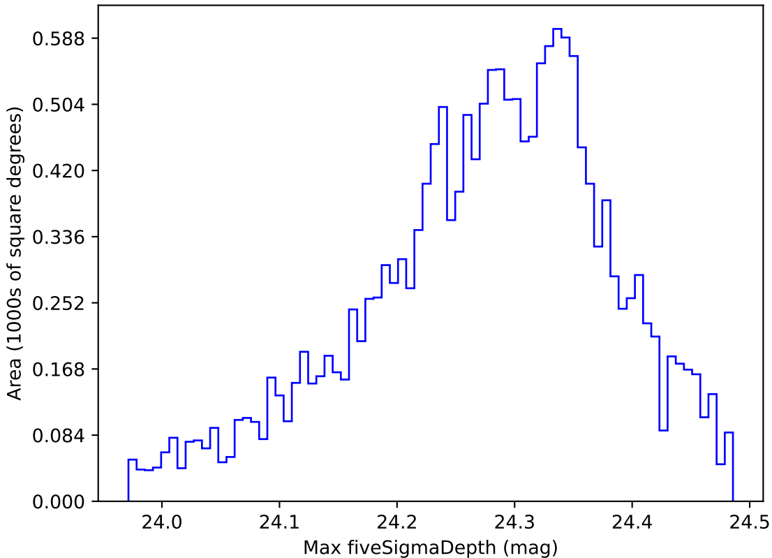
ddf_loaded_fl1_v3.4_10yrs WFD i band: Max fiveSigmaDepth
